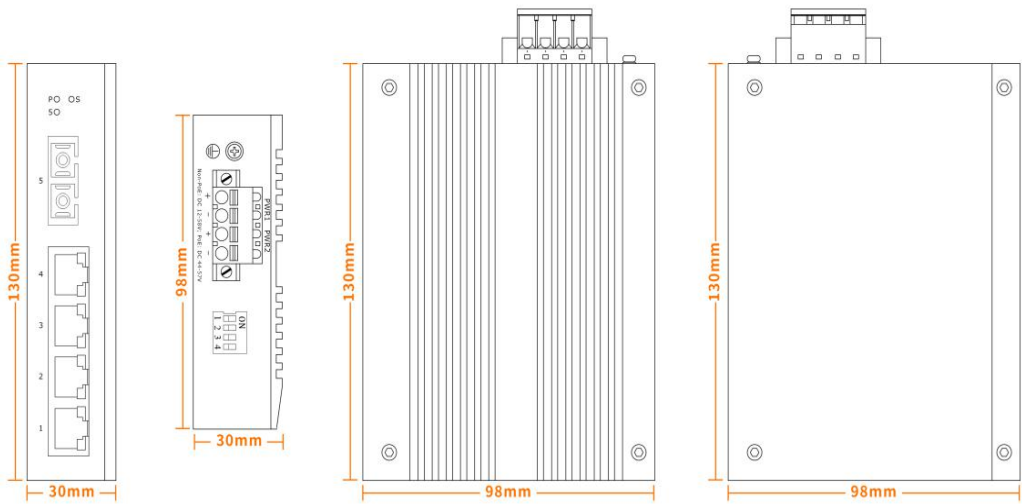
SC/ST/FC model
