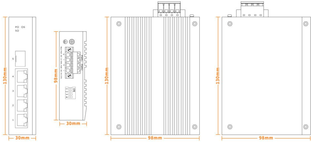
SFP model
